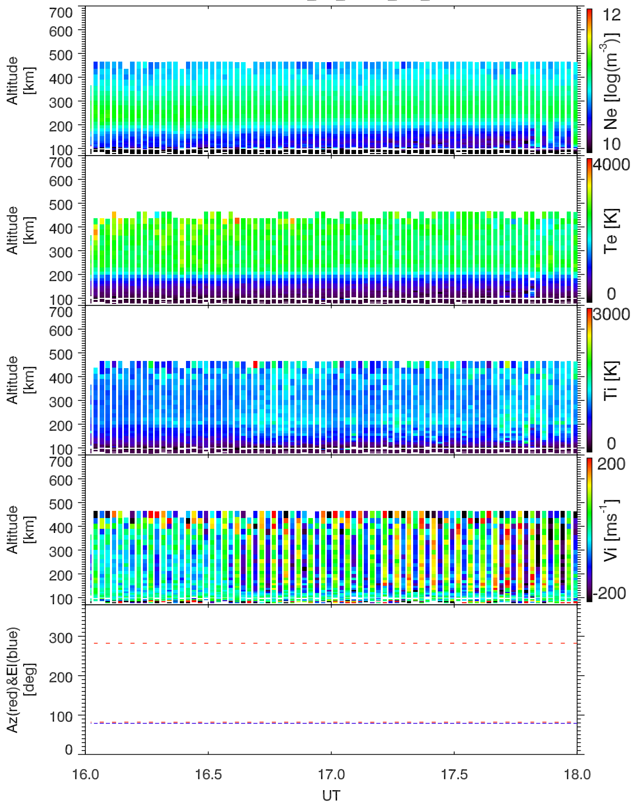
EISCAT 2007-04-04_16_18UT_ipy_ant@32m.
