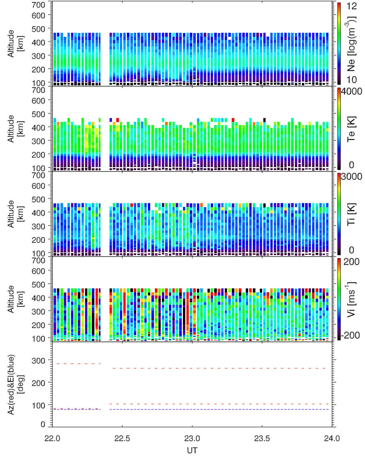
EISCAT 2007-04-26_22_24UT_ipy_ant@32m.
