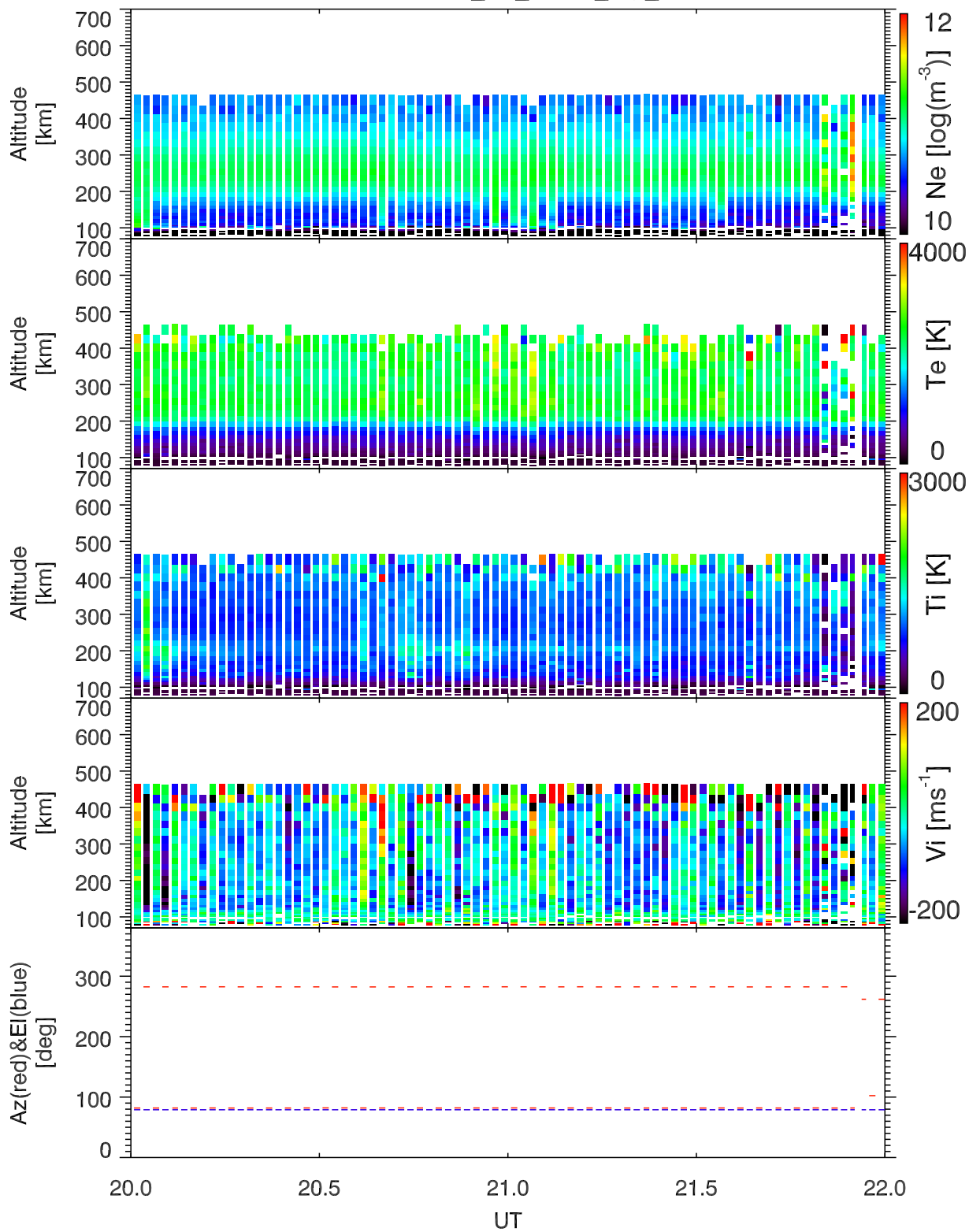
EISCAT 2007-05-10_20_22UT_ipy_ant@32m.
