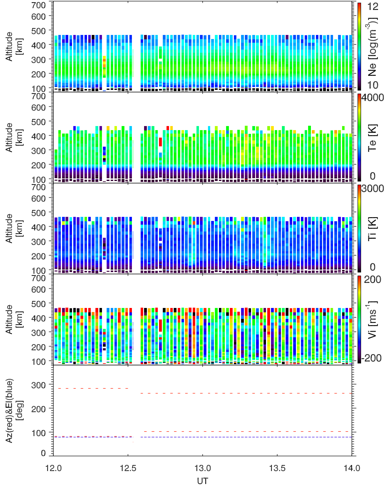
EISCAT 2007-09-14_12_14UT_ipy_ant@32m.
