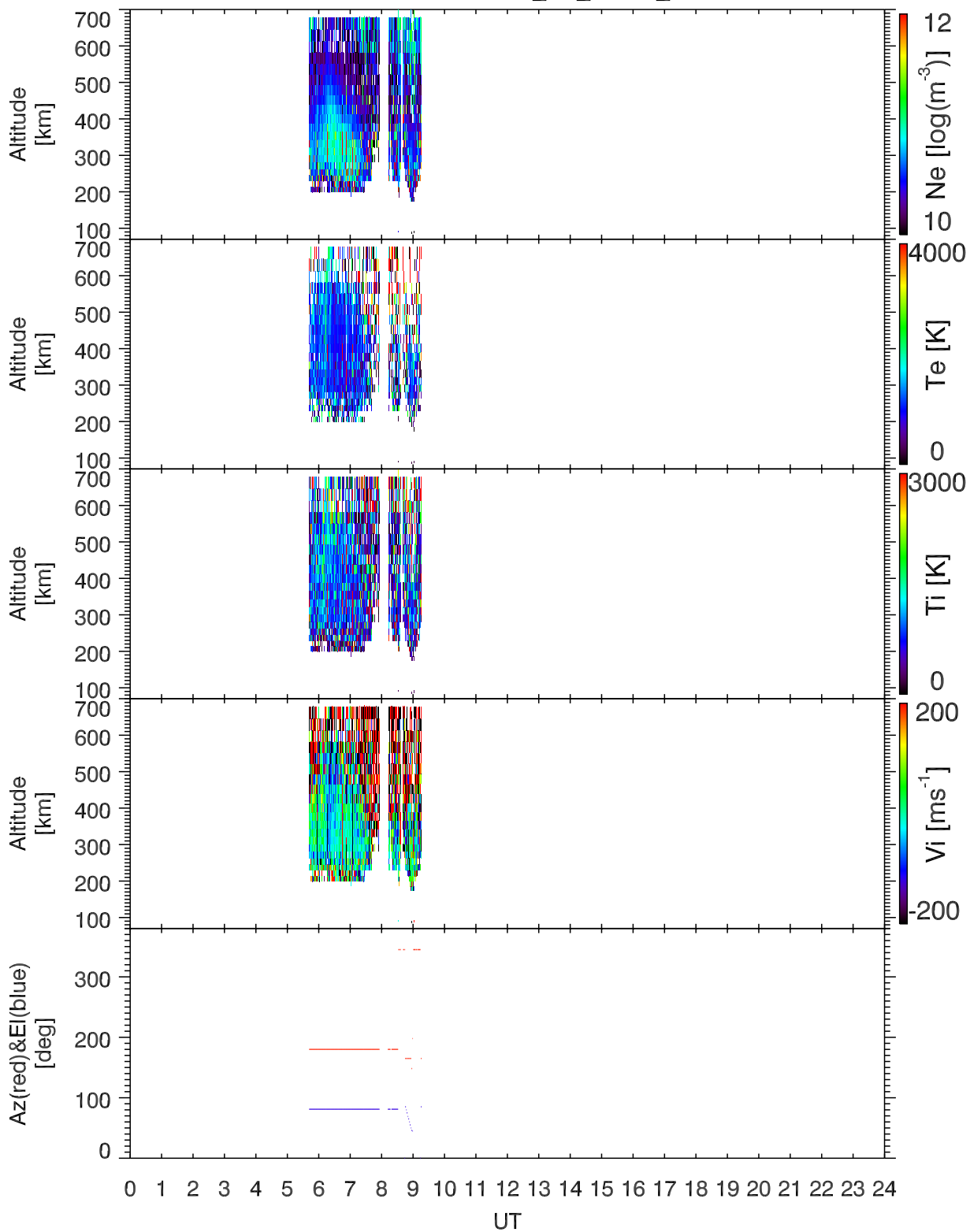
EISCAT 1997-12-01_00_24UT_32m
