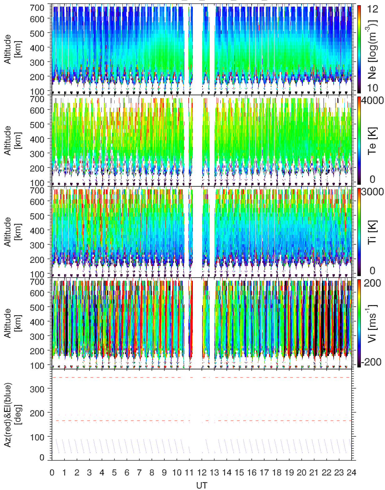
EISCAT 1998-04-28_00_24UT_gup0_ant@32m.
