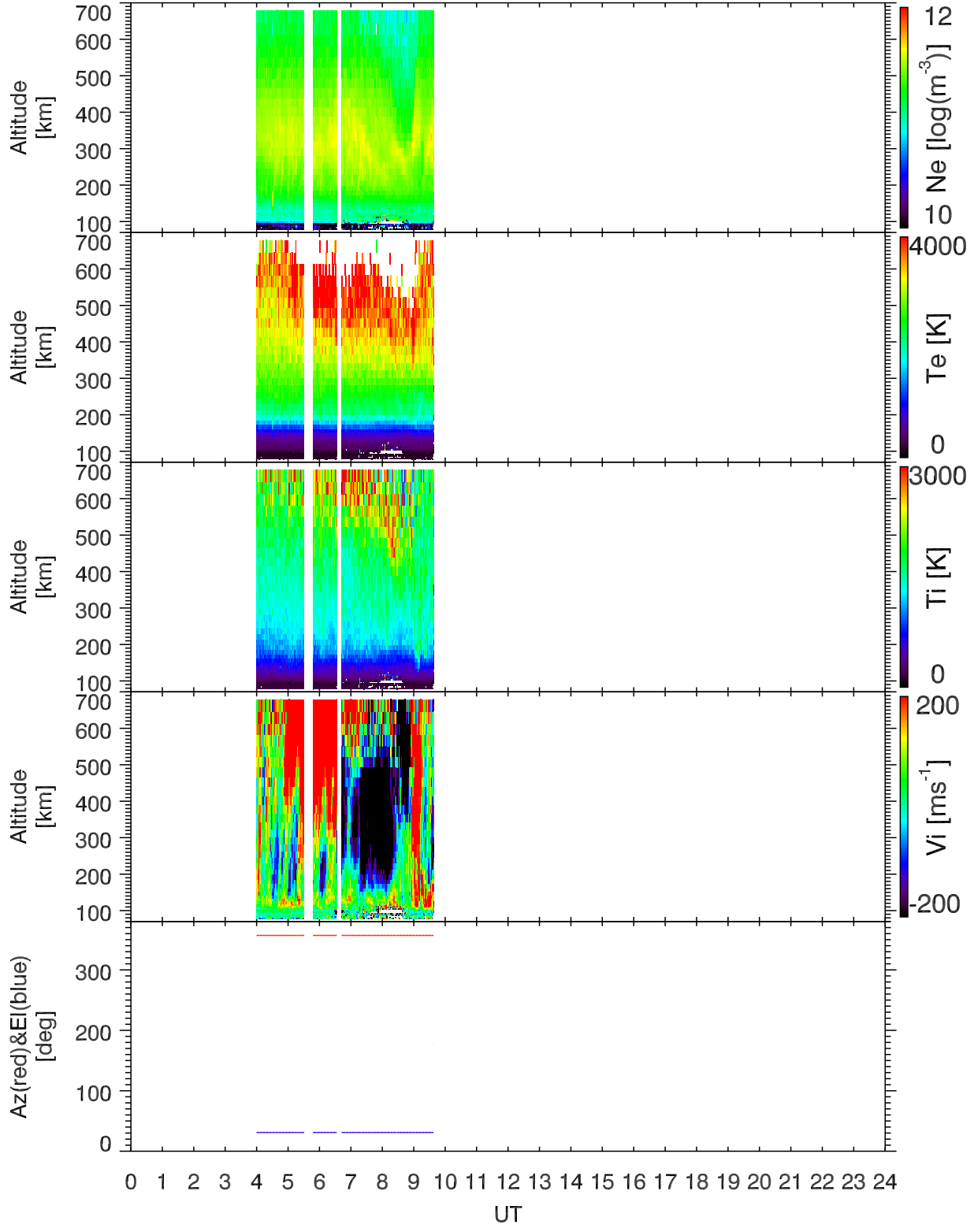
EISCAT 2000-07-17_00_24UT_tau0_120@32m.
