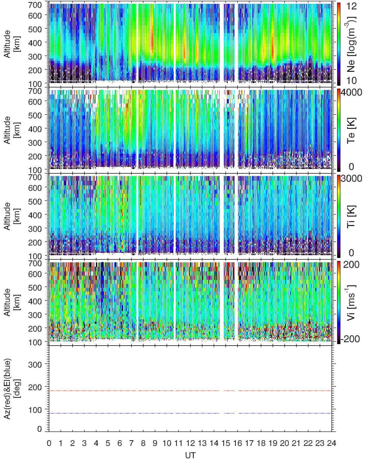
EISCAT 2001-12-13_00_24UT_tau0_120@42m.
