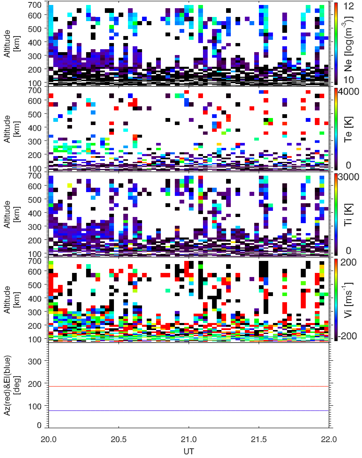
EISCAT 2008-11-05_20_22UT_beata_120@uhfa.
