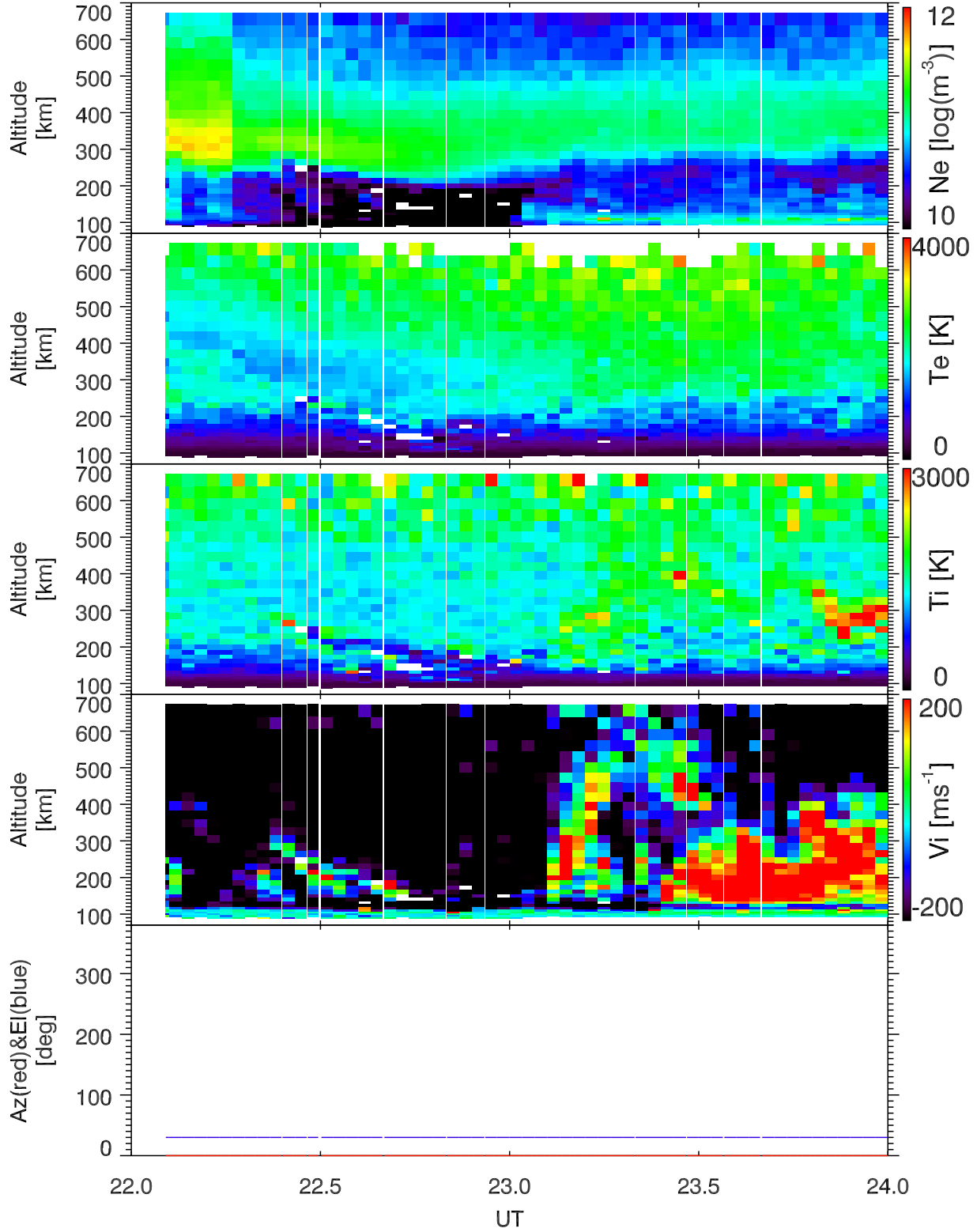
EISCAT 2001-04-16_22_24UT_tau1a_120@vhfa.
