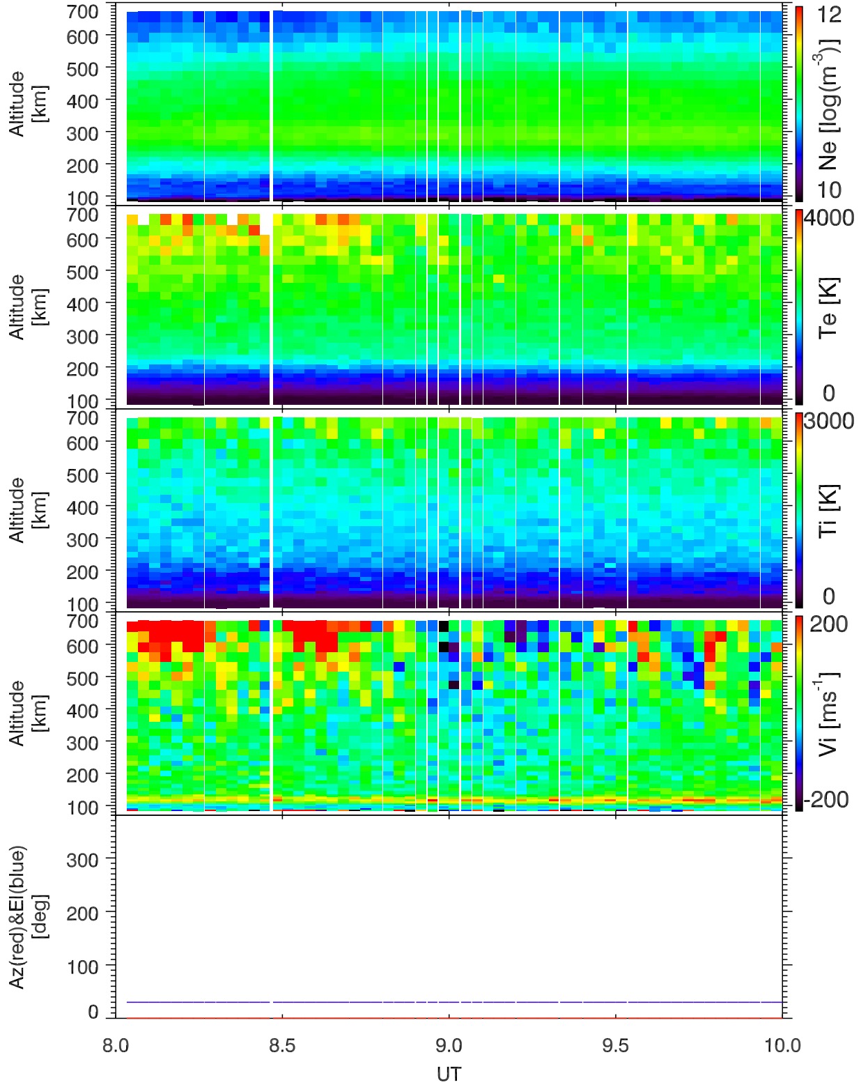
EISCAT 2001-04-17_08_10UT_tau1a_120@vhfa.
