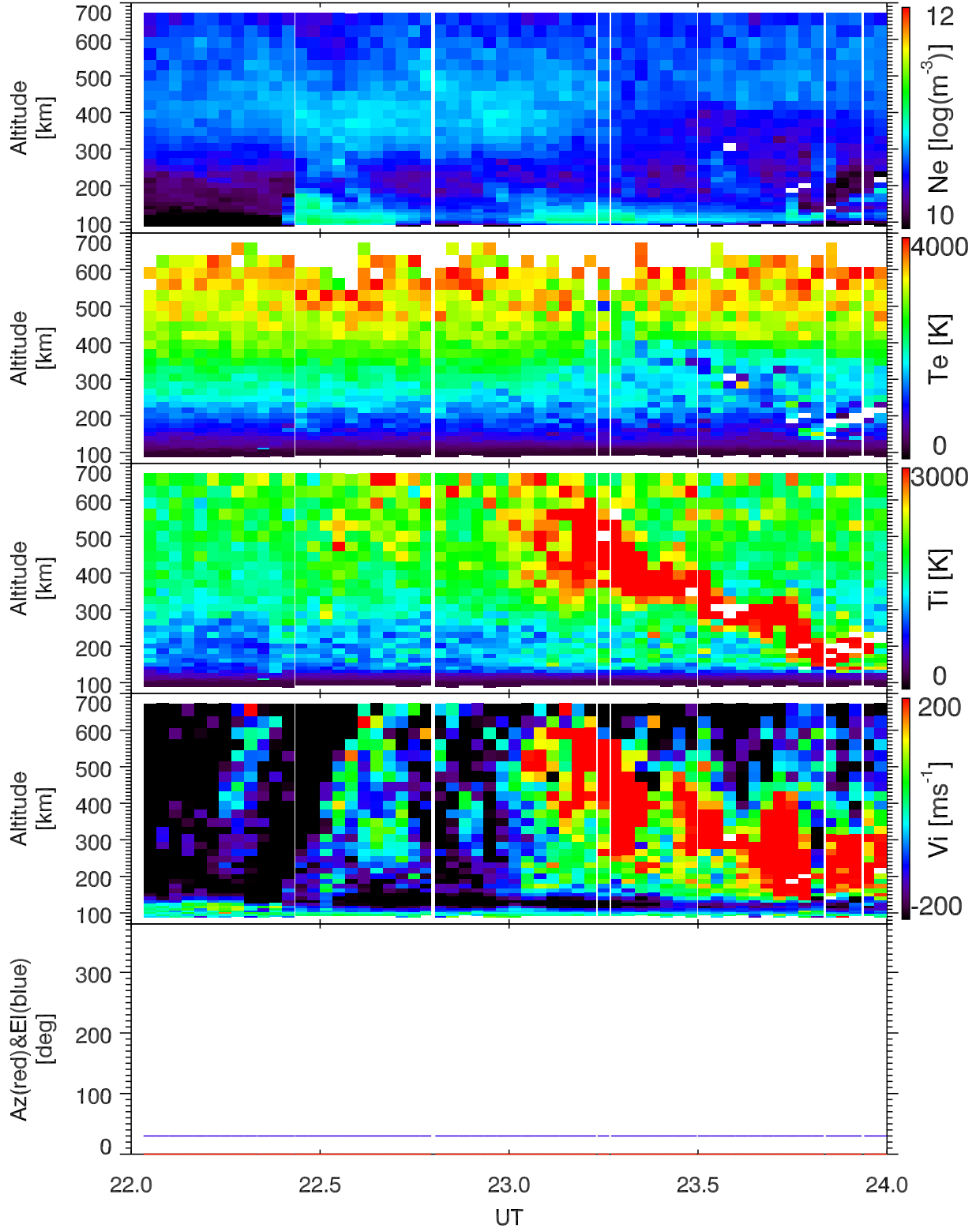
EISCAT 2001-04-28_22_24UT_tau1a_120@vhfa.
