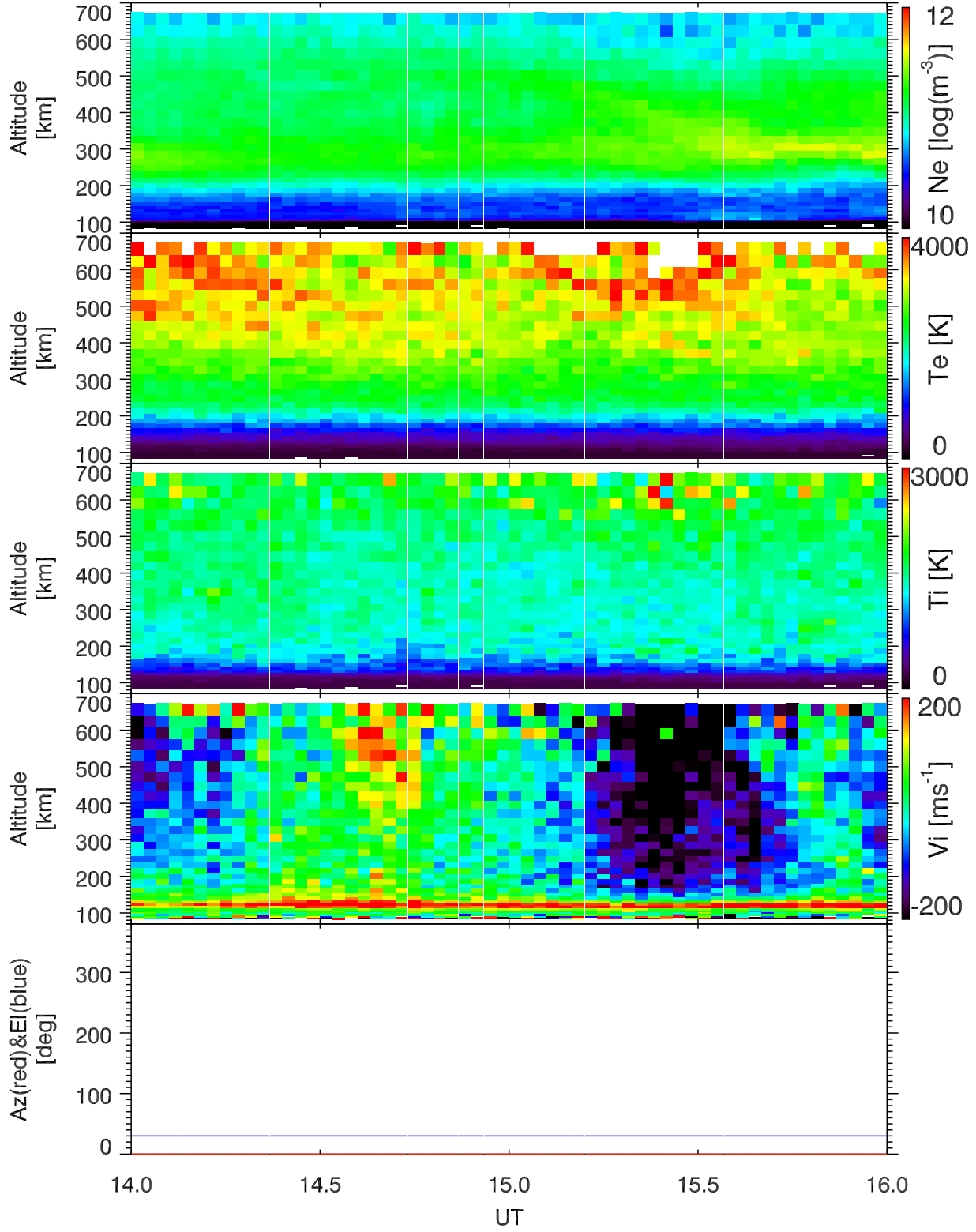
EISCAT 2001-09-11_14_16UT_tau1a_120@vhfa.
