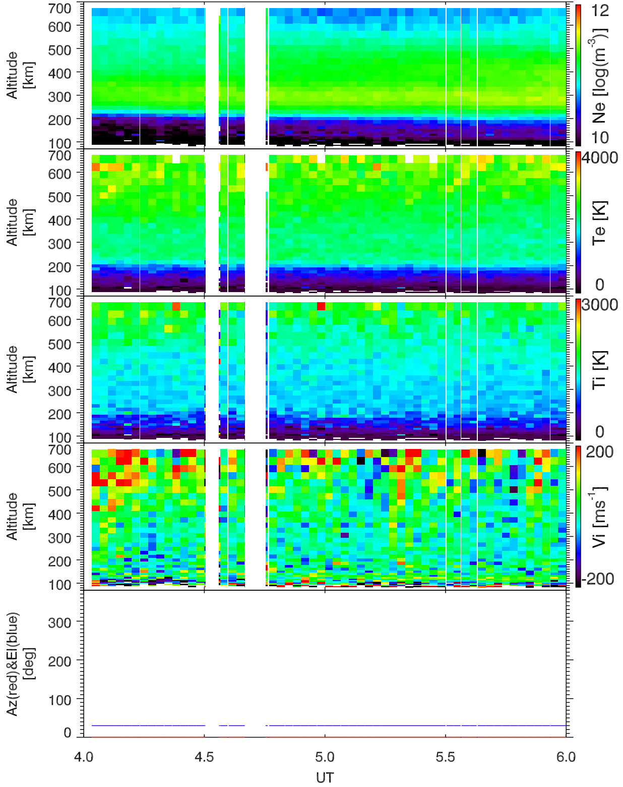
EISCAT 2001-09-21_04_06UT_tau1a_120@vhfa.
