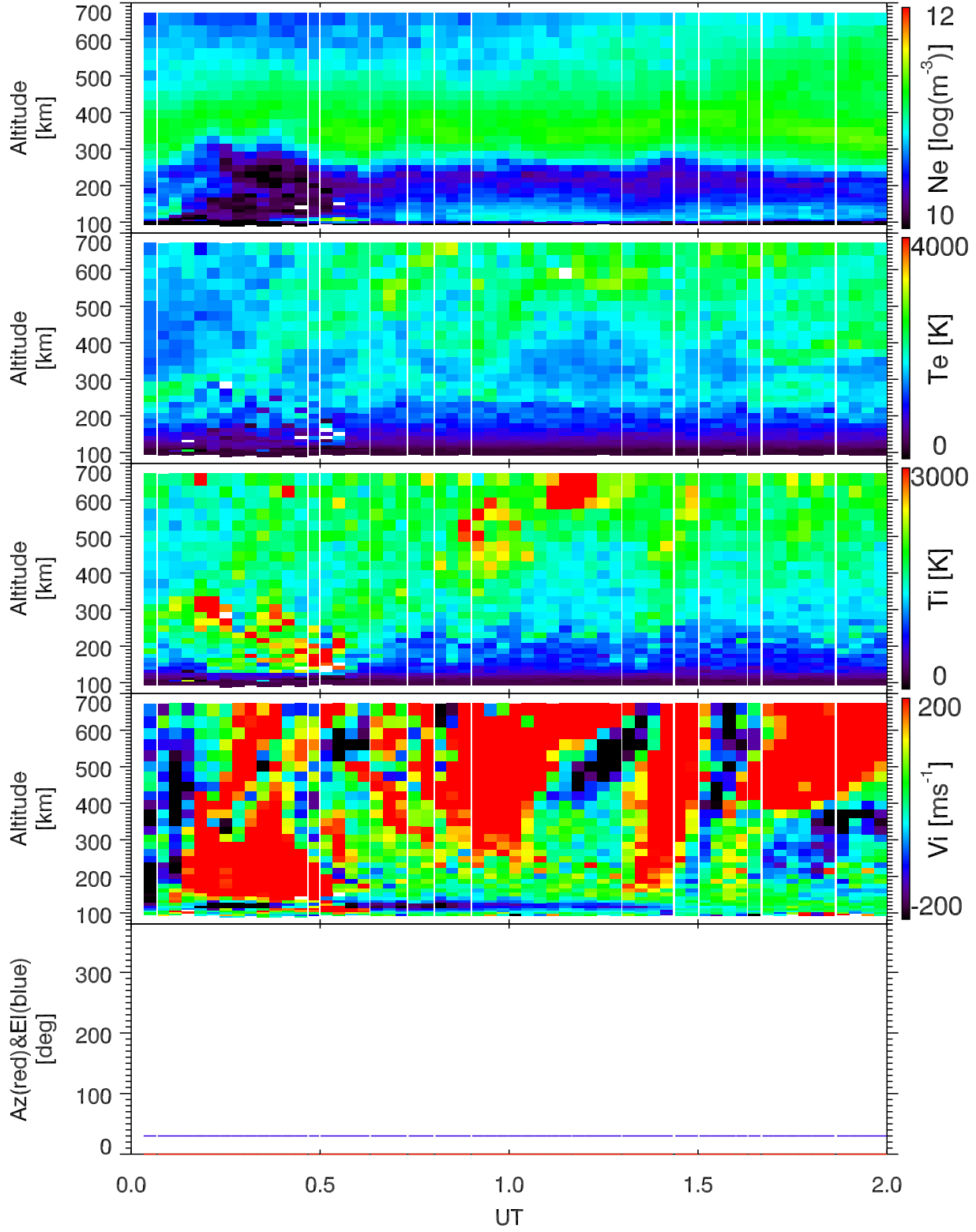
EISCAT 2001-09-22_00_02UT_tau1a_120@vhfa.
