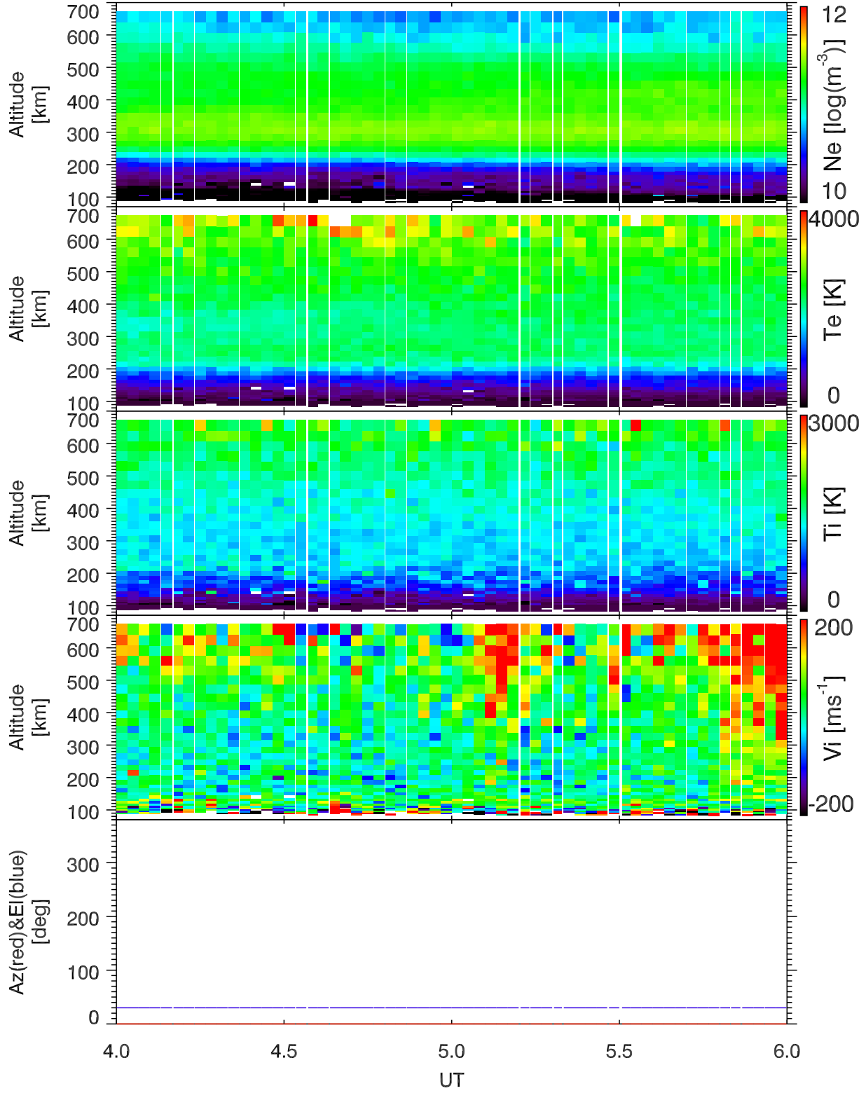
EISCAT 2001-09-22_04_06UT_tau1a_120@vhfa.
