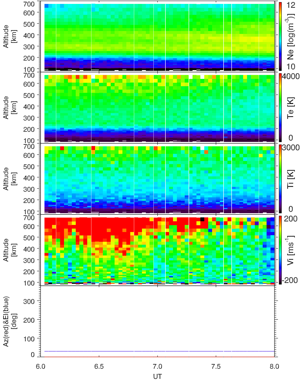
EISCAT 2001-09-22_06_08UT_tau1a_120@vhfa.
