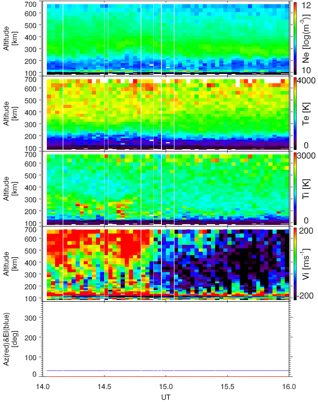
EISCAT 2001-09-22_14_16UT_tau1a_120@vhfa.
