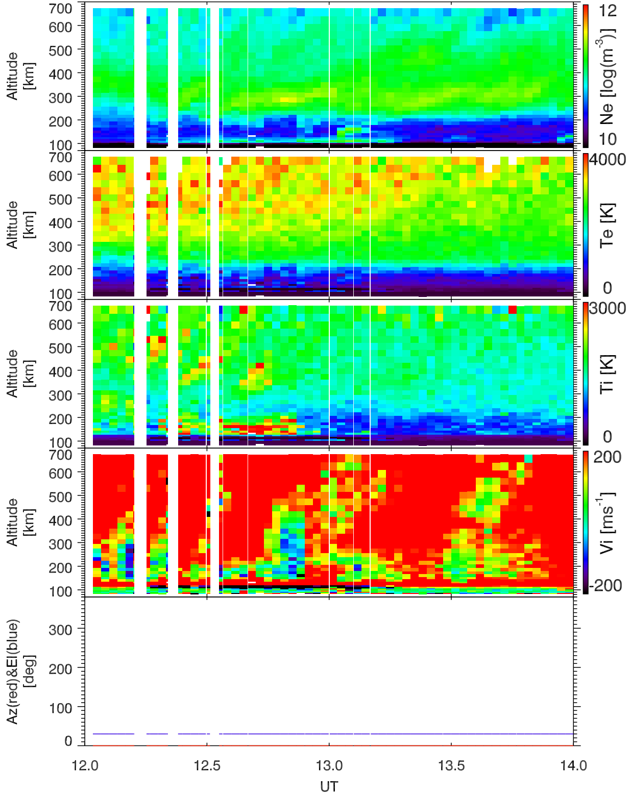
EISCAT 2001-10-09_12_14UT_tau1a_120@vhfa.
