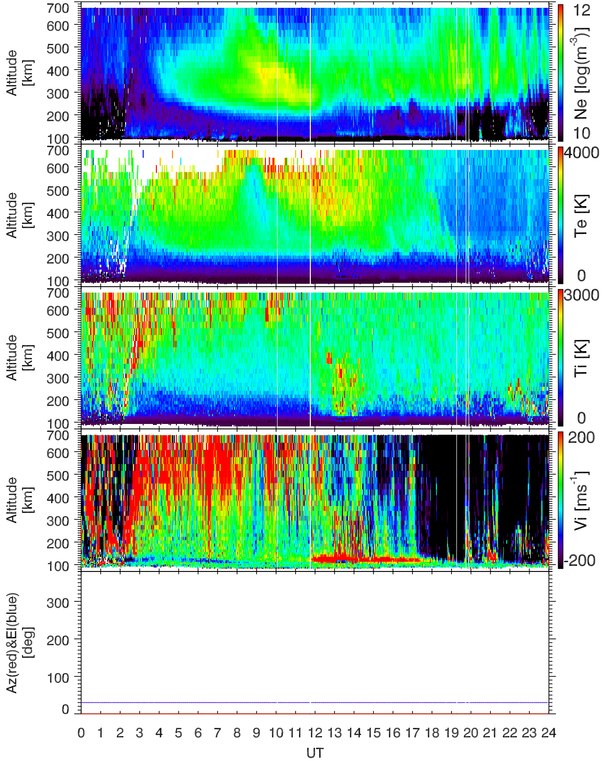
EISCAT 2001-10-10_00_24UT_tau1a_120@vhfa.
