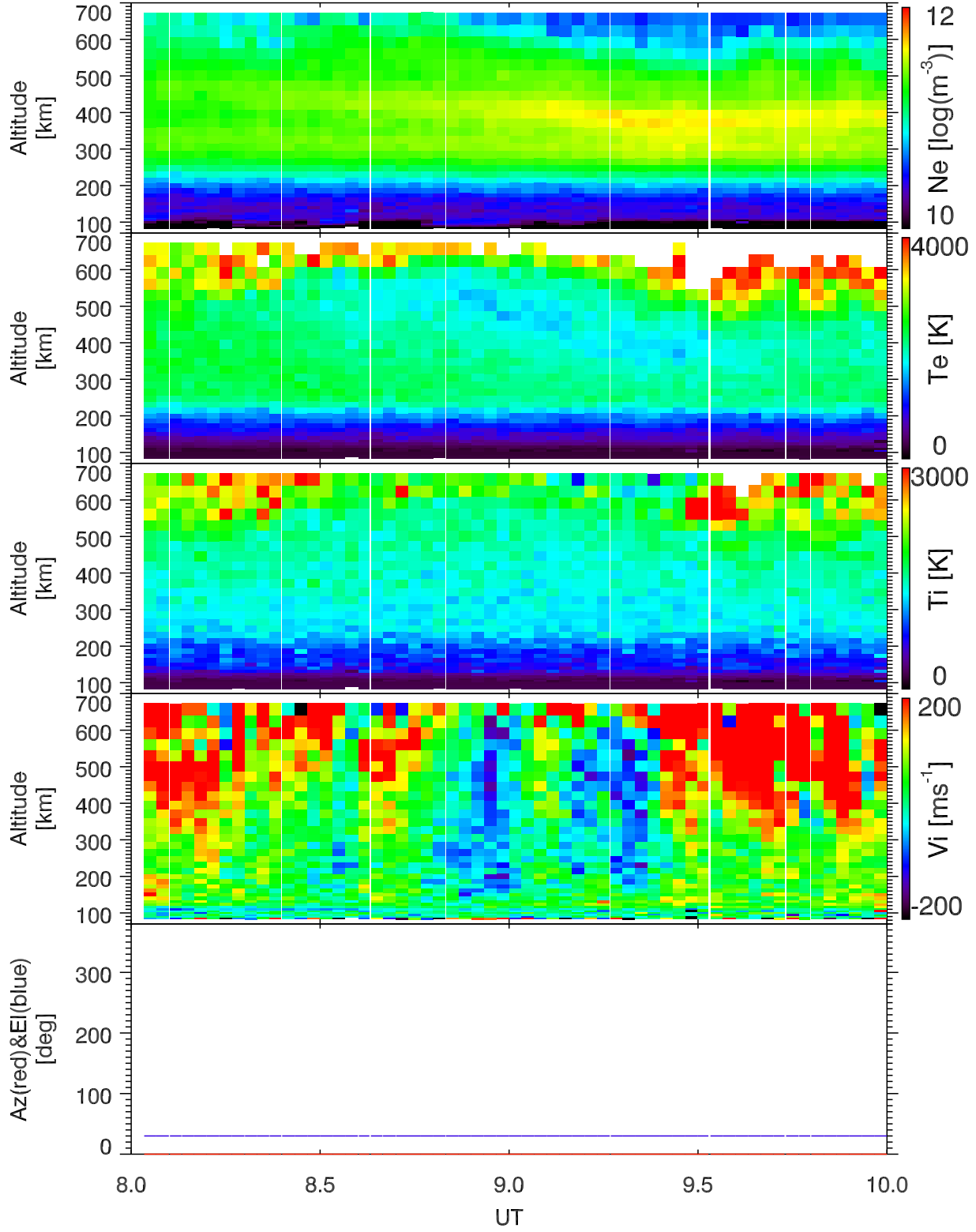
EISCAT 2001-10-10_08_10UT_tau1a_120@vhfa.
