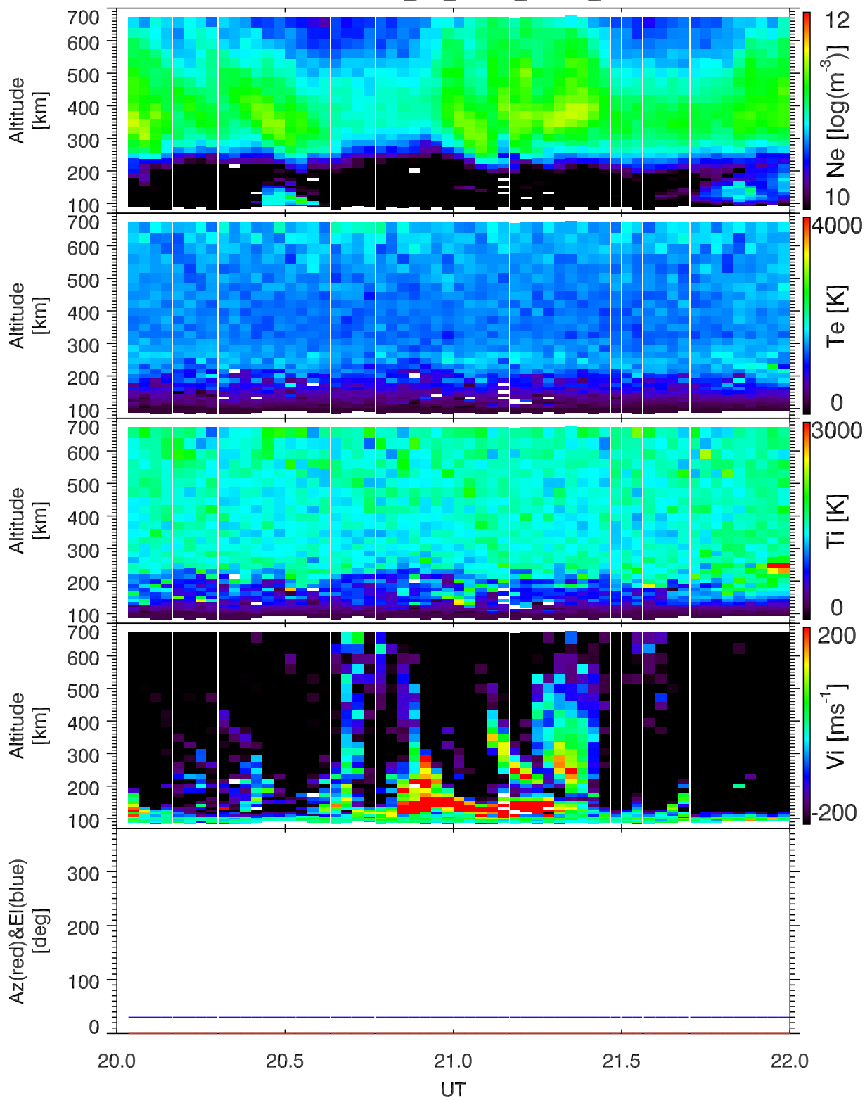
EISCAT 2001-10-10_20_22UT_tau1a_120@vhfa.
