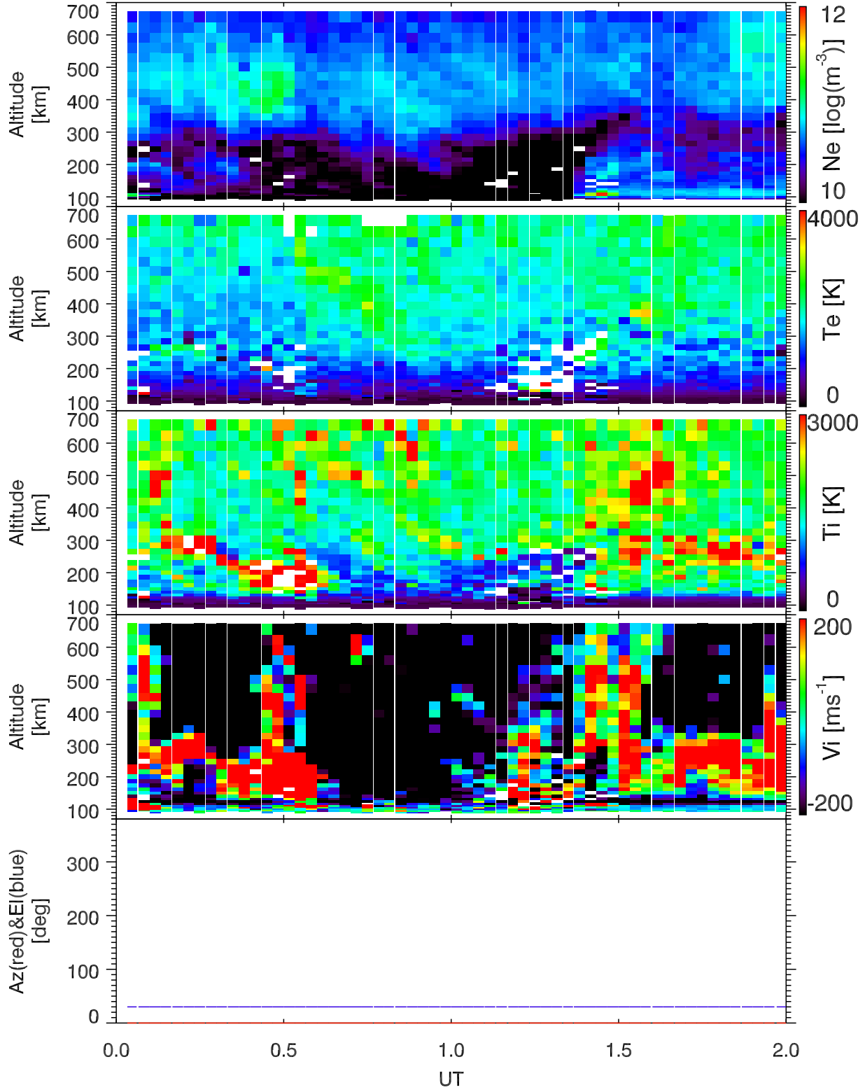
EISCAT 2001-10-11_00_02UT_tau1a_120@vhfa.
