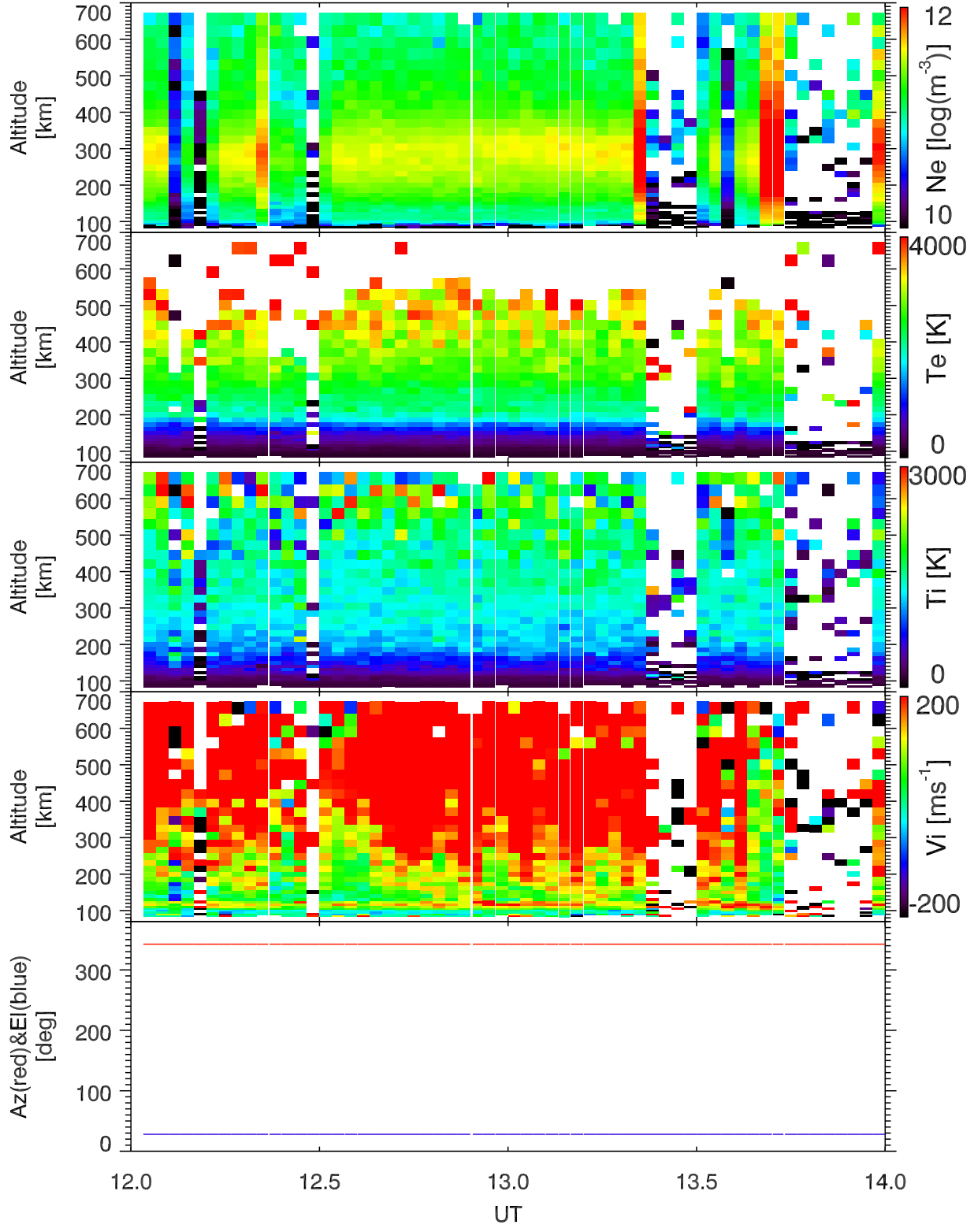
EISCAT 2002-08-13_12_14UT_tau1a_120@vhfb.
