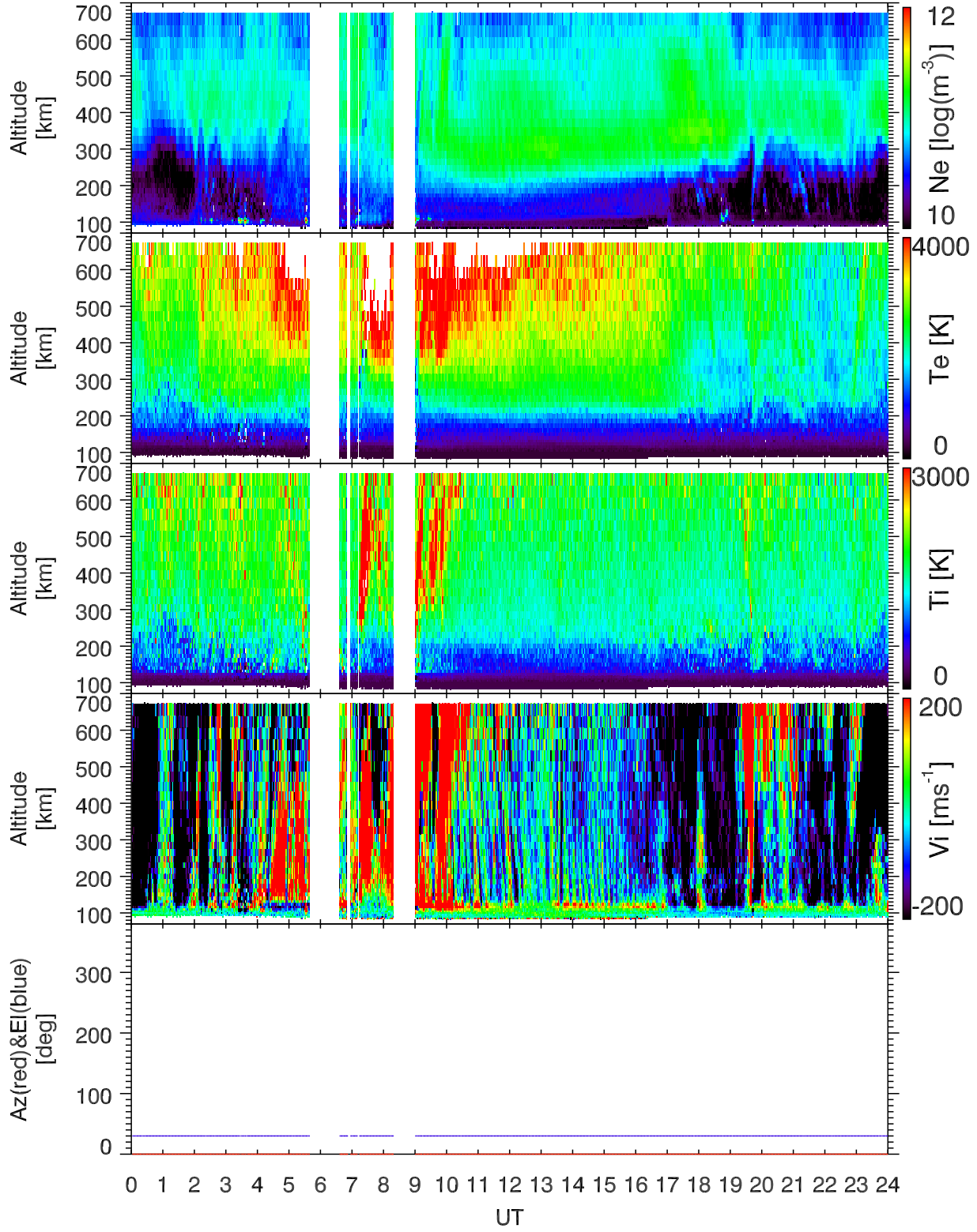
EISCAT 2001-09-26_00_24UT_tau1a_120@vhfa.
